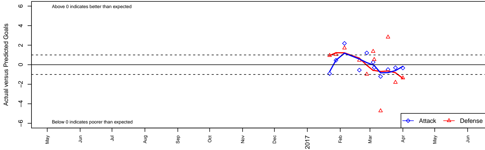
STU Chelsea Academy B03 Dots are actual minus expected GF (blue circles) and GA (red triangles). Blue line is smoothed change in attack strength. Red is smoothed change in defense strength.
